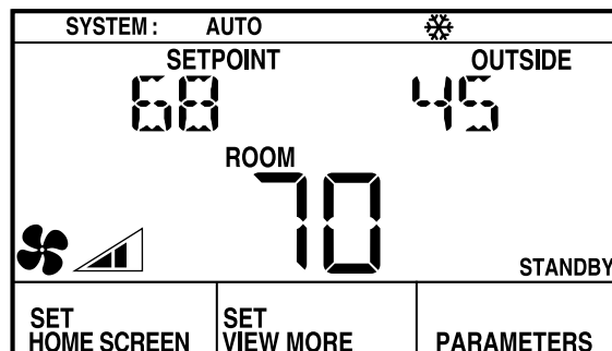
Fig. 7. Sample Contractor Home screen display with System Status, Setpoint, Outside Temperature, and Room Temperature (predominant).
