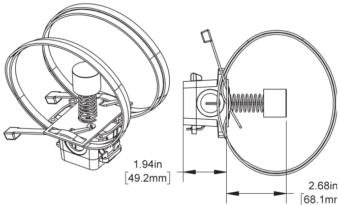
Spring-Loaded Strap BAPI-Box Crossover (BBX)
