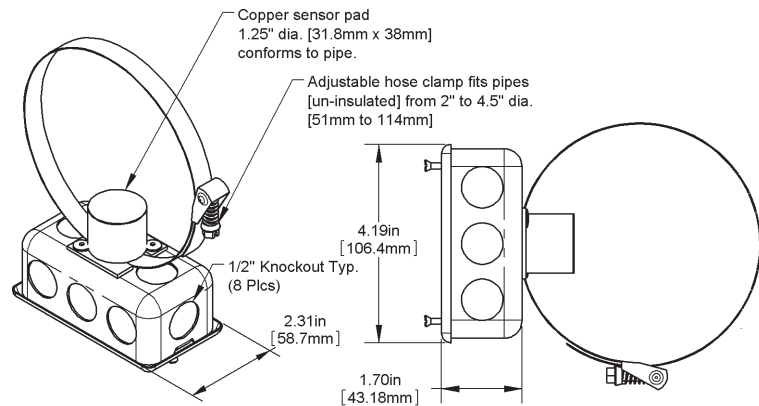
Clamp-On Strap Junction Box (JB)
